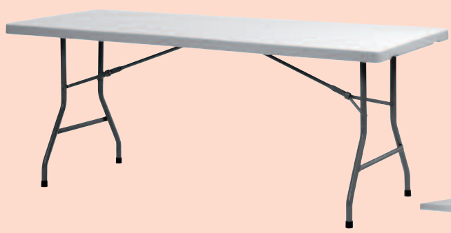
XXL240 TABLE L.2400 × W.914 × H.743 mm
